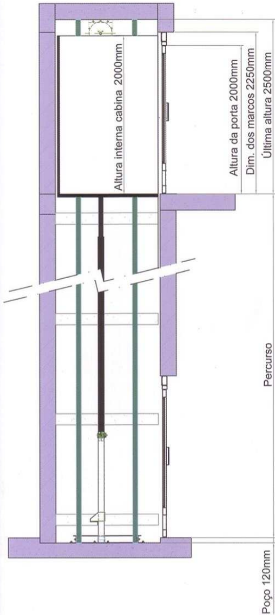
Corte Vertical
